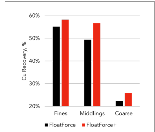
Cu recovery of first rougher cell
