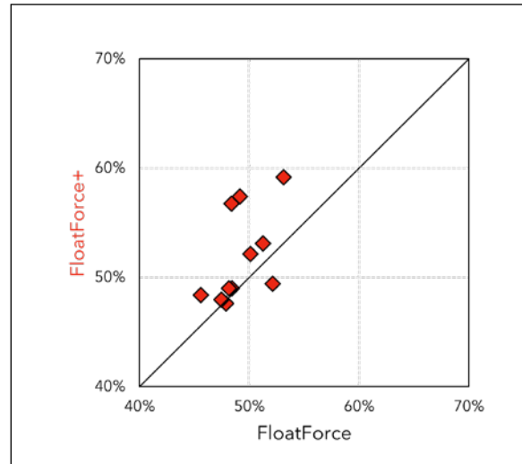
FloatForce+ vs FloatForce Cu recovery
